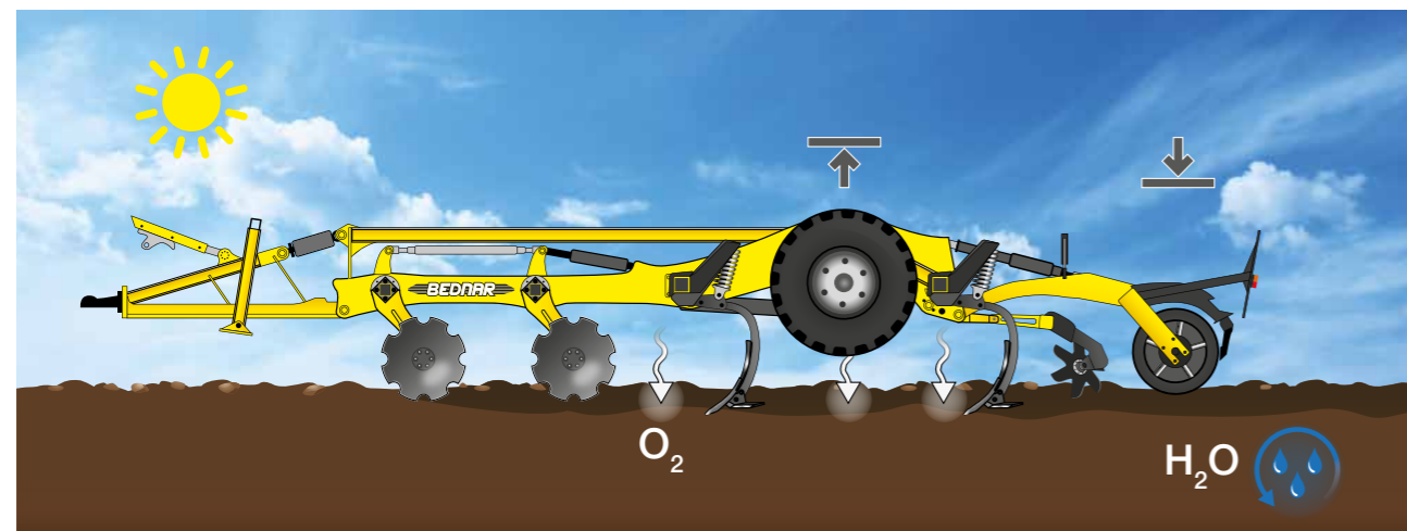
Loosening with compaction (driving on rollers)
